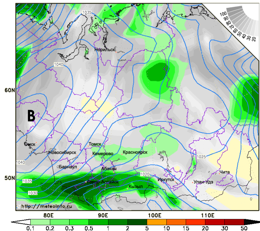
03:00 15.11.2019 (MCK) MSLP, precipitation and cloudiness 13.11.2019 00 UTC + 048h
