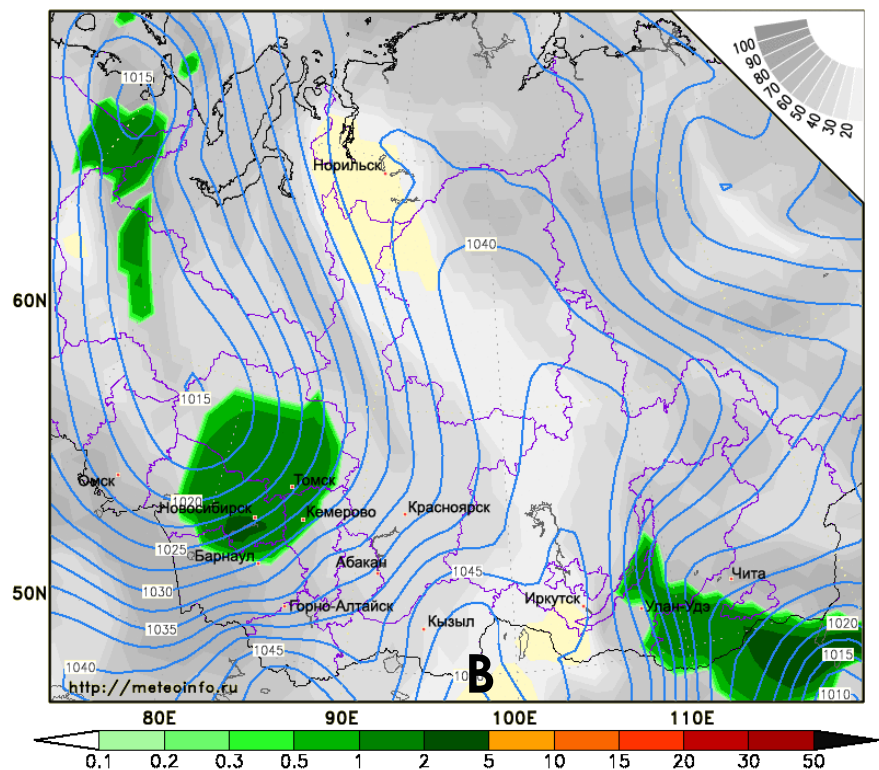
03:00 17.11.2019 (МСК) MSLP, precipitation and cloudiness 13.11.2019 00 UTC + 096h
