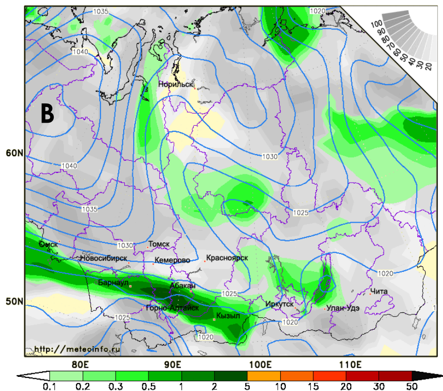
03:00 14.11.2019 (MCK) MSLP, precipitation and cloudiness 13.11.2019 00 UTC + 024h
