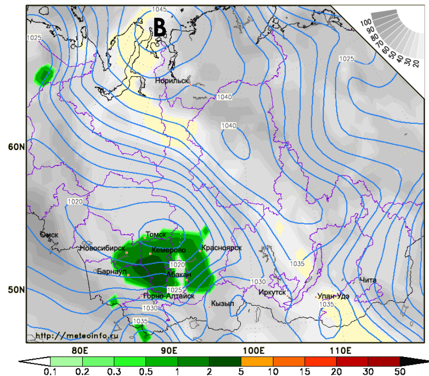
03:00 18.11.2019 (МСК) MSLP, precipitation and cloudiness 13.11.2019 00 UTC + 120h
